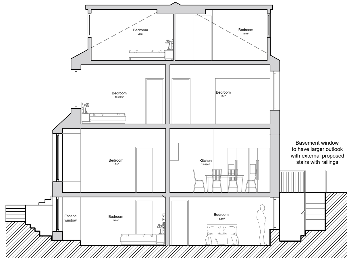
PROPOSED SECTION B 1:100 @ A3 (showing internal changes)
